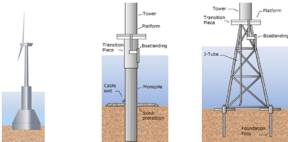
Figur 3.4 Eksempler af fundamenterstyper (set fra venstre side): gravitationsfundamenter; monopæl; Jacket-type fundamenter (kilde: https://www.obayashi.co.jp/chronicle/130th/en/archives/chapter4_1_5.html# oraz: https://www.researchgate.net/figure/Three-types-of-tur
